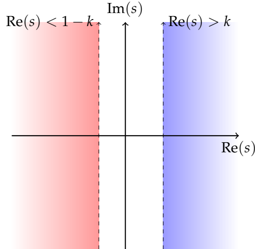
Figure 5.4 The domain of D(s, \sigma_k) .
