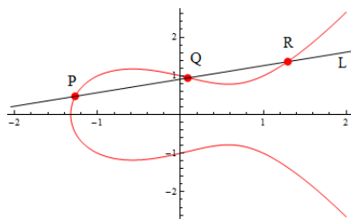
Figure 1.2 Step 2 of the Operation for elliptic curves: Identifying R = P \oplus Q .
