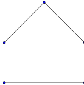
Figure 4.2 A cycle graph on 5 vertices
