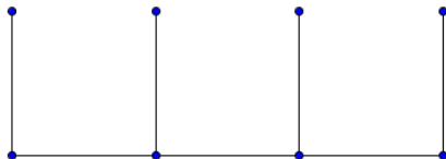
Figure 4.4 A 4-centipede graph
