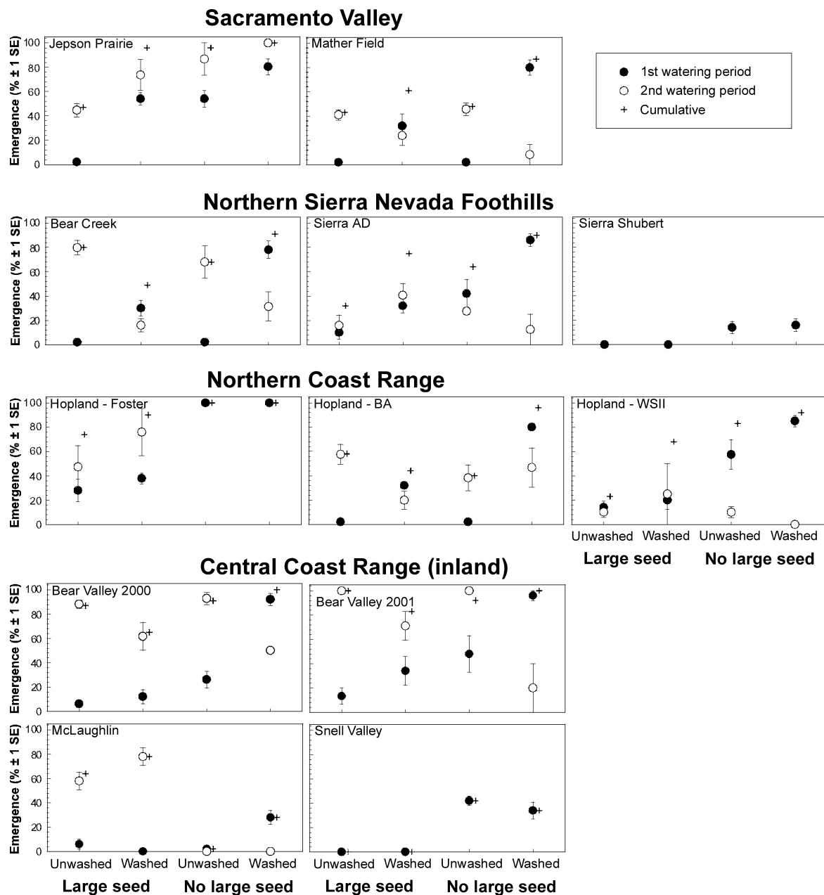
Fig. 2.—Effects of washing of spikelets and the presence of large seeds on the emergence ( \% \pm 1 \text{ SE} ) of small seeds of Aegilops triuncialis for 12 populations representing four sampled regions. The first wet period stimulated complete germination of the large seeds (when present). Maternal and sibling effects were predicted to be strongest in the first watering period (filled circles) and weaker in the second period (open circles). Although washing and large seed removal treatments did have significant effects on emergence, the responses varied strongly among populations (see Table 2).
