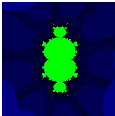
(b) z^3 + c ( d = 3 )
