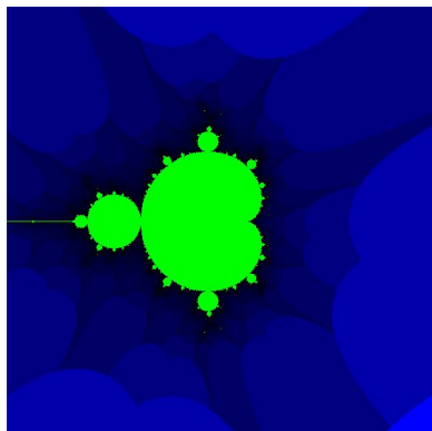
(a) z^2 + c ( d = 2 )
