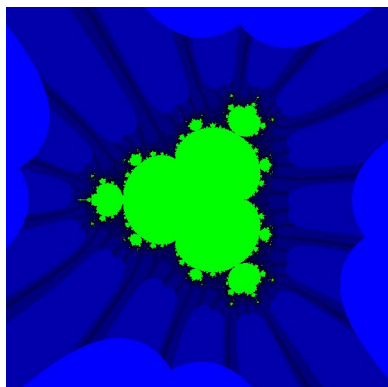
(c) z^4 + c ( d = 4 )
