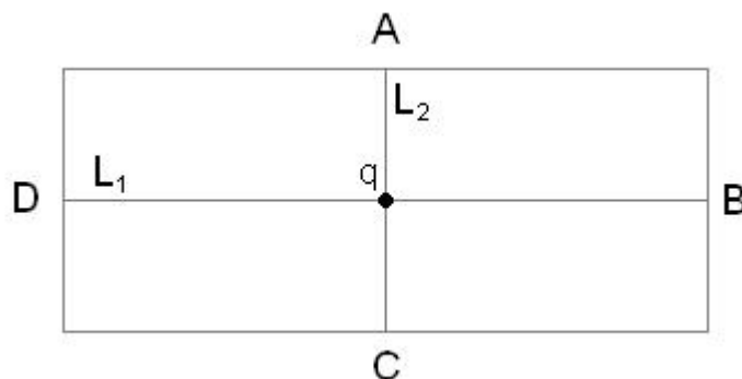
Figure 2.1: A non-square rectangle has no conformal center.
