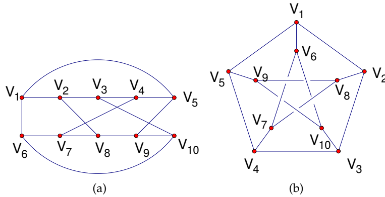
Figure 3.10: Five crossedges on two cycles of length five isomorphic to the Petersen graph.
