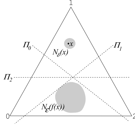
Figure 2.2: An example where Cohen’s labelling does not guarantee that the limit point of the completely-labelled simplices is a fixed point.
