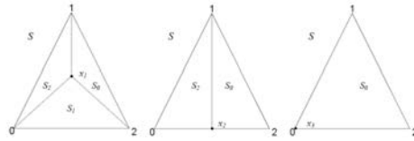
Figure 3.1: The construction of the simplices S_i(t) 's, when S is a 2-dimensional simplex.
