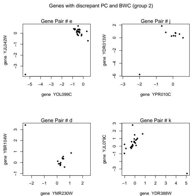
Figure 2 Each point represents the \log_2(R/G) value for the specified genes on a particular array. The Pearson correlation and the biweight correlation give opposite values for these group 2 pairs. Due to the outlying values, it is clear that the Pearson correlation is quite misleading.
