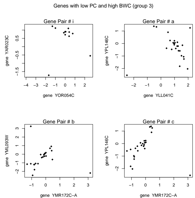
Figure 3 Each point represents the \log_2(R/G) value for the specified genes on a particular array. The Pearson correlation is close to zero, and the biweight correlation gives a relatively high value for these group 3 pairs.
