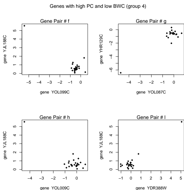
Figure 4 Each point represents the \log_2(R/G) value for the specified genes on a particular array. The biweight correlation is close to zero, and the Pearson correlation gives a high absolute correlation. Group 4 pairs are the most worrisome; it would be a mistake to think that two genes were highly correlated when that high correlation is simply due to one outlying point.
