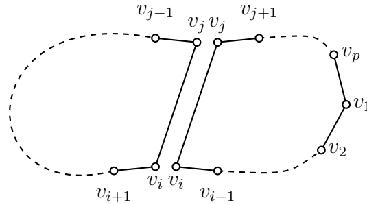
Figure 3: Splitting the graph over a chord from v_i to v_j
