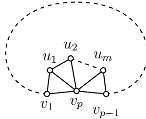
Figure 4: Neighbors of the vertex v_p
