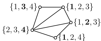
Figure 2: An example of coloring from lists
