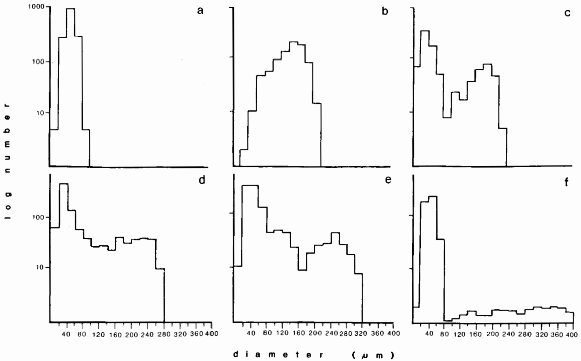
Fig. 1. Distribution of vessels by diameter in six species of deciduous trees: a) Acer pennsylvanicum ; b) Juglans cinerea ; c) Fraxinus americana ; d) Carya tomentosa ; e) Quercus rubra ; and f) Q. macrocarpa .
