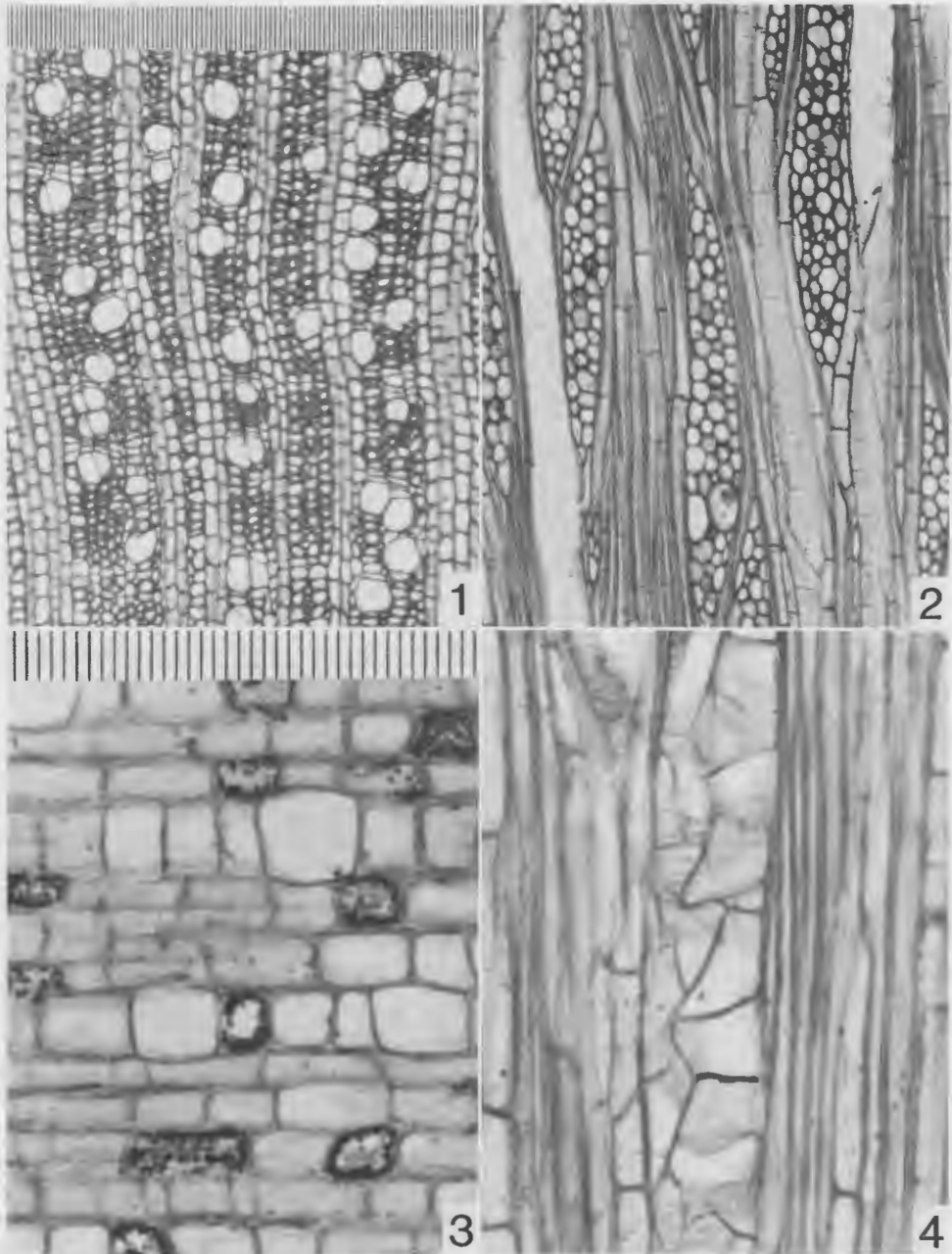
Fig. 1-4. Wood sections of Degeneria roseiflora (Miller 1200).—1. Transection; vessels are relatively narrow, fiber-tracheids thick walled.—2. Tangential section; two etherial oil cells in ray, bottom center; two uniseriate rays near lower left corner.—3. Radial section; enlarged cells are etherial oil cells; dark-staining droplets restricted to certain other cells.—4. Radial section; tyloses in vessel, center. (Fig. 1-2, magnification scale above Fig. 1 [finest divisions = 10 \mu\text{m} ]; Fig. 3, 4, scale above Fig. 3 [divisions = 10 \mu\text{m} ].)
