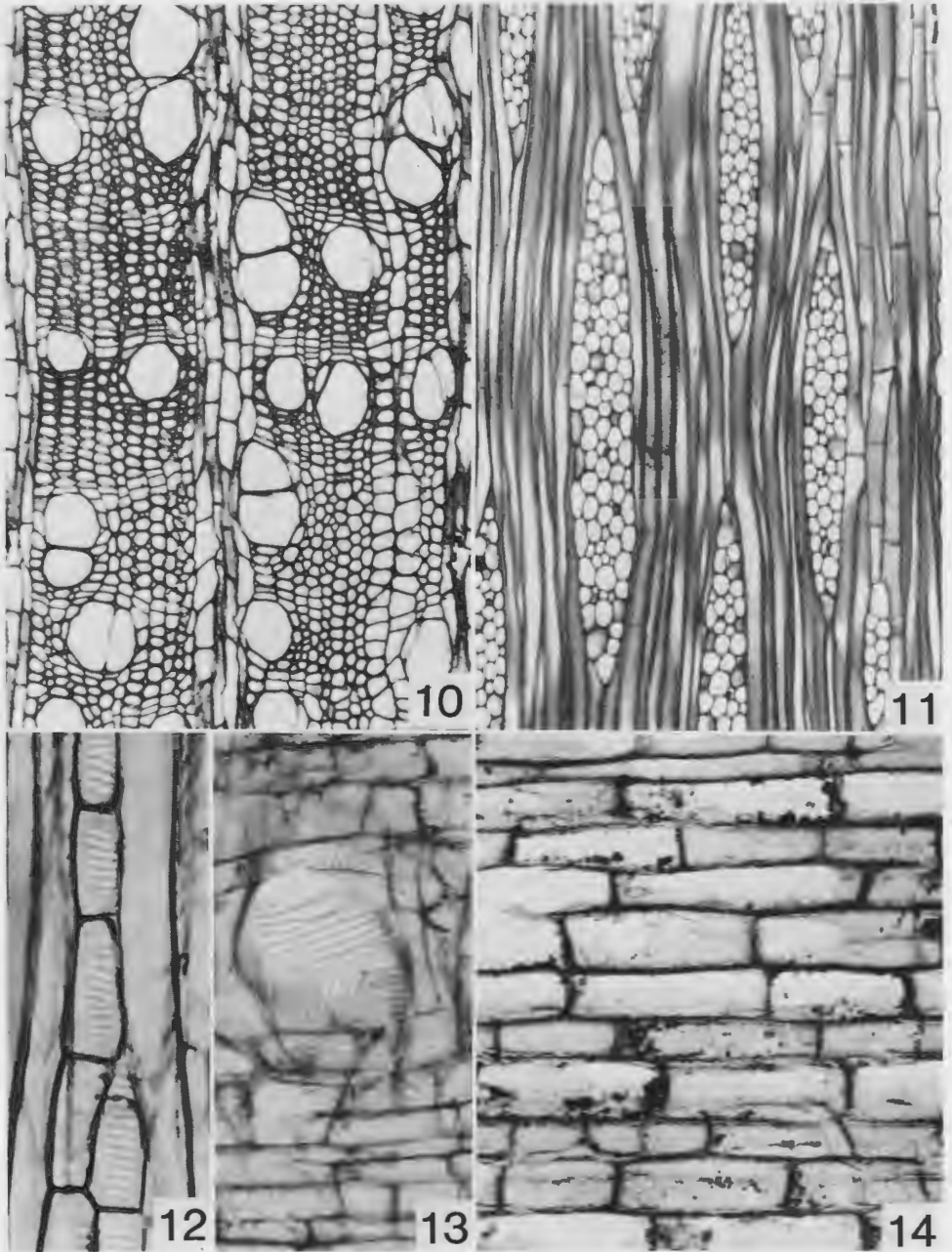
Fig. 10–14. Wood sections of Degeneria vitiensis (SFCw-R 1193-1).—10. Transection; vessels are relatively wide, fiber-tracheids thin walled.—11. Tangential section; rays are all multiseriate.—12. Radial section; scalariform vessel-axial parenchyma pitting.—13. Radial section; perforated ray cell with scalariform perforation plate.—14. Radial section; ray cells are all markedly procumbent; some contain dark-staining droplets. (Fig. 10, 11, magnification scale above Fig. 1; Fig. 12–14, scale above Fig. 3.)
