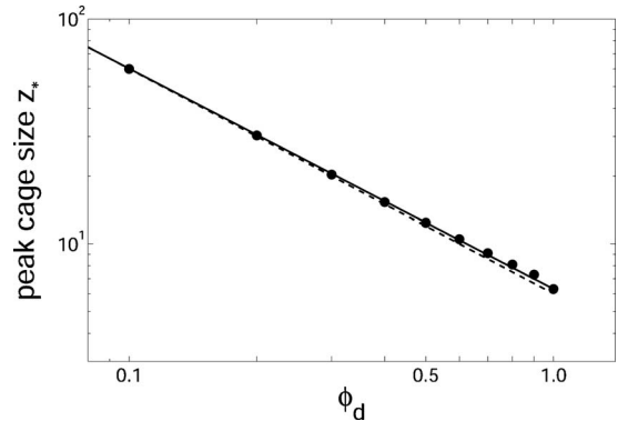
FIG. 4. The peak cage size z_* as a function of dimer concentration \phi_d . The solid line is the best-fit power law, as described in the text. The dotted line is the theoretical prediction z_* = 6/\phi_d , which ignores correlations between dimer orientations. Error bars derived from counting statistics are comparable to the marker size.
