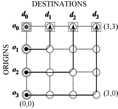
Figure 3: The only nonintersecting 4-route for the digraph given in Figure 1 is associated with the identity permutation. Thus the determinant equals 1.
