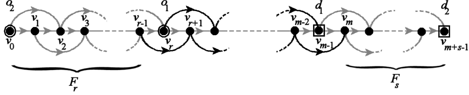
Figure 5: The directed graph associated with Cassini's generalized Fibonacci determinant, F_{m-r}F_{m+s} - F_mF_{m+s-r} = (-1)^{m+1-r}F_rF_s . The black arcs are required in a nonintersecting 2-route.
