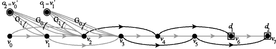
Figure 7: The Gibonacci digraph \mathcal{G}_7(\{0, 1\}) associated with Cassini's Gibonacci identity.
