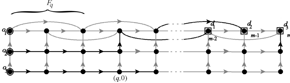
Figure 10: The 3 \times m binomial digraph plus the arcs ((i, 2), (i+2, 2)) for 0 \leq i \leq m-2 .
