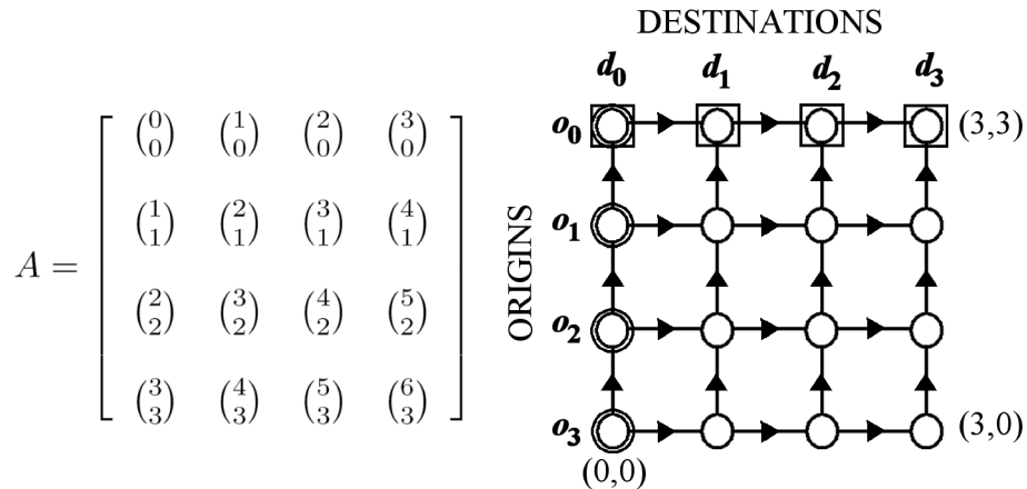
Figure 1: The 4 \times 4 binomial matrix and its associated directed graph. Origin nodes are enclosed by a circle and destination nodes are enclosed by a square.
