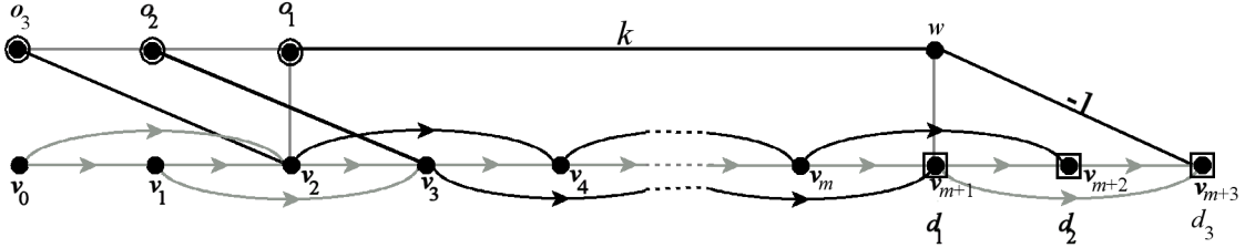
Figure 11: Adding vertices and weighted arcs to the Fibonacci digraph changes the determinant.
