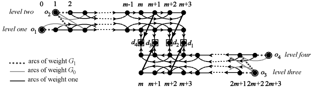
Figure 18: This digraph is used to prove equation (17). The arcs exiting each origin have weight G_0 or G_1 as indicated above.
