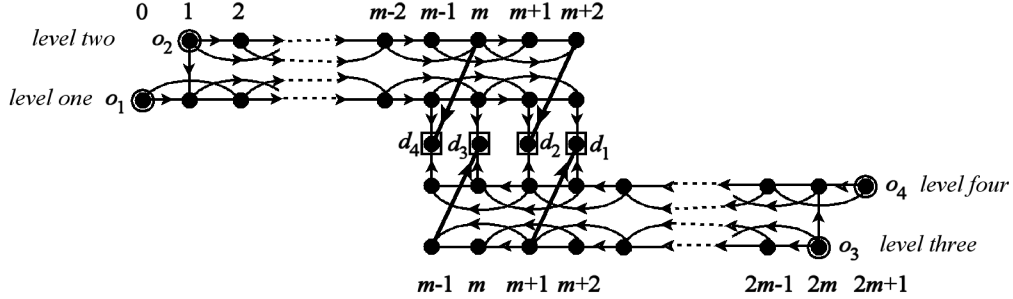
Figure 14: This digraph is used to prove equation (16). For convenience, unlabeled vertices will be referred to by position. So v_{s,r} is the vertex in column s on level r .
