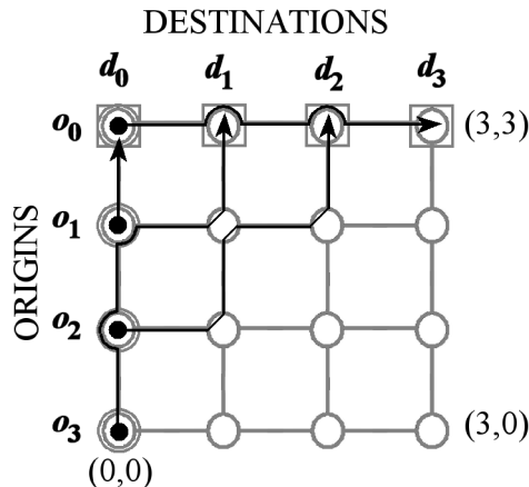
Figure 2: One of the eighteen 4-routes associated with the permutation (031)(2) .
