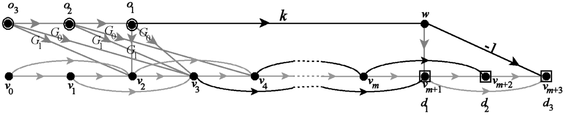
Figure 12: Adding weighted arcs to the Gibonacci digraph. The black arcs are required in a nonintersecting 3-route.
