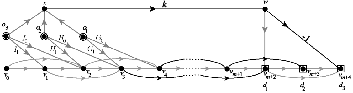
Figure 13: A more intuitive and more general digraph than Figure 12. The black arcs are required in all nonintersecting 3-routes.
