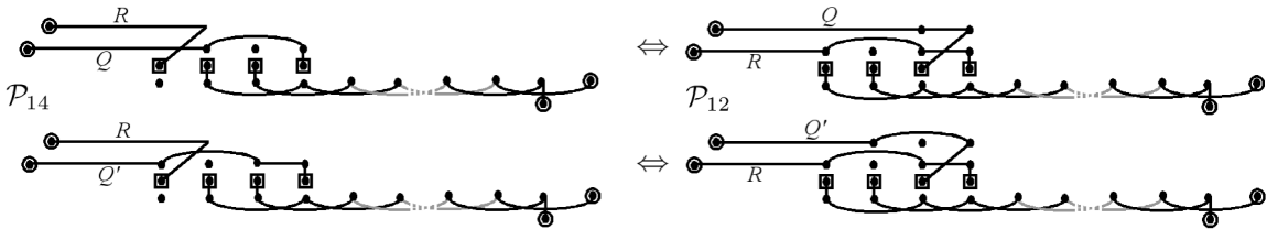
Figure 17: Illustrating the bijections between members of \mathcal{P}_{14} where the level one path does not end and members of \mathcal{P}_{12} where the level one path does not pass through vertex v_{m,1} .
