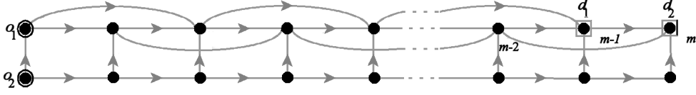
Figure 9: The digraph \mathcal{H}_m contains the 2 \times m binomial digraph plus the arcs ((i, 1), (i + 2, 1)) for 0 \leq i \leq m - 2 .
