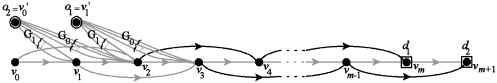
Figure 8: The directed graph associated with Cassini's generalized Gibonacci determinant, G_{m-1}G_{m+1} - G_m^2 = (-1)^{m-1}(G_0G_2 - G_1^2) . The black arcs are required in a nonintersecting 2-route.
