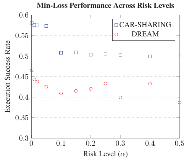
Figure 4: MIN-LOSS DC execution success rate across different risk levels ( \alpha ). Generally, MIN-LOSS DC performed at its best when risk was minimized.
