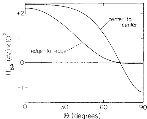
FIG. 11. H_{BA} as a function of \Theta for (0, \pi) states. a , b , V_0 , and E are as in Fig. 9 for the (0, \pi) states. Shown are results for a constant center-to-center distance of 10 \text{ \AA} and for a constant edge-to-edge distance of 5 \text{ \AA} .
