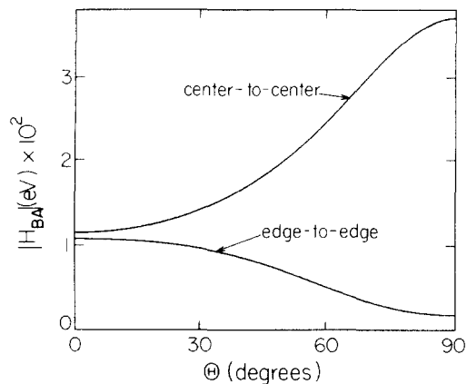
FIG. 10. |H_{BA}| as a function of \Theta for a pair of (0, \sigma) states. a , b , V_0 , and E are as in Fig. 9 for the (0, \sigma) states. Shown are results for a constant center-to-center distance of 10 \text{ \AA} and for a constant edge-to-edge distance of 5 \text{ \AA} .
